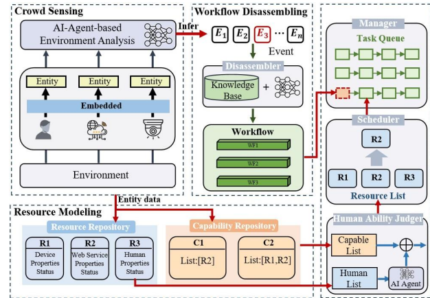
Figure 1: System architecture of Scenario-Driven CPSS.
