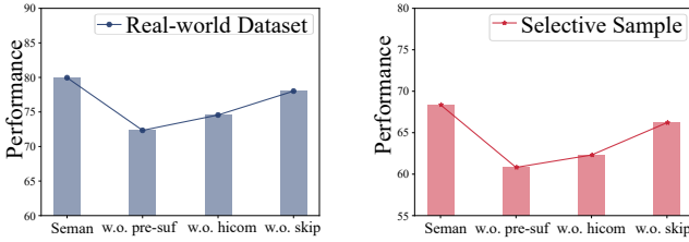
Figure 5: Ablation Study. We design three variants of Samen and compare their performance on raw Yelp (left) and sample set with concept shift (right).
