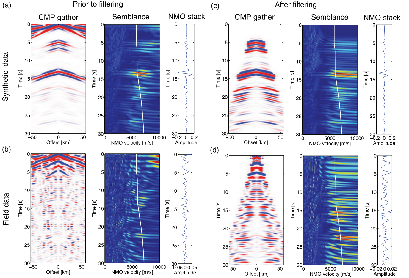
Figure 7. A common-midpoint gather, retrieved with seismic interferometry, for the midpoint position coinciding with station 12 (left-hand panel), its semblance (middle panel) and normal-move-out stack (right-hand panel), using the model velocity function v_p(t) as depicted by the white line in the semblance plot (middle panel). The same three panels are shown for the synthetic data (a), the field data (b) and the synthetic and field data after filtering, (c) and (d), respectively.
