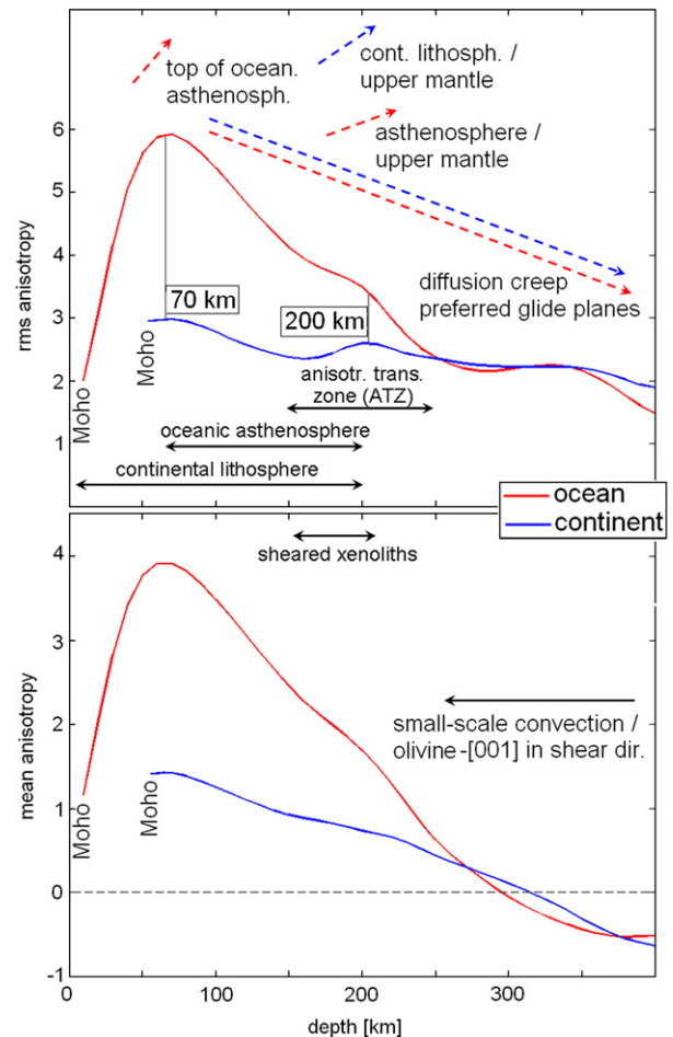
Fig. 8. Horizontal averages of the rms (top) and mean (bottom) radial anisotropy, (v_{sh} - v_{sv})/v_{sv}^{iso} as a function of depth. The averages are over the continental (blue solid curve) and oceanic (red solid curve) regions with non-zero ray coverage. Dashed arrows are qualitative indicators of the different contributions that lead to increasing (upward pointing) or decreasing (downward pointing) anisotropy beneath the continent (blue) and the ocean (red). Black arrows mark the approximate depth intervals of the continental lithosphere, the oceanic asthenosphere, the anisotropic transition zone (ATZ), the region where sheared xenoliths originate, and the region where small-scale convection and the alignment of the olivine [001] axis in the direction of shear are expected.
