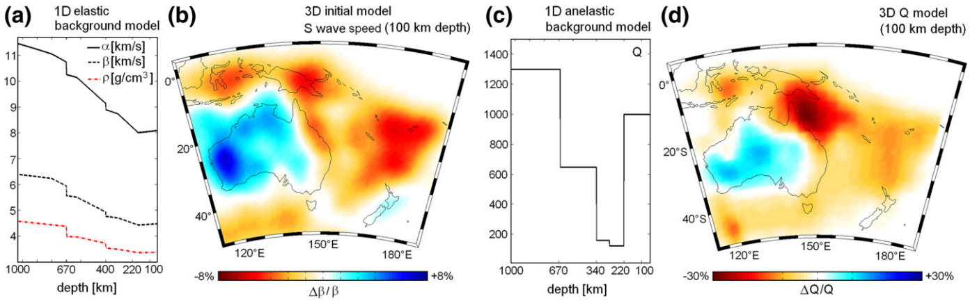
Fig. 1. Left panels: (a) 1D elastic background model of the P wave speed, \alpha , the S wave speed, \beta , and density, \rho . (b) Horizontal slice at 100 km depth through the initial 3D S wave speed model. Right panels: (c) 1D background model of shear attenuation. (d) Horizontal slice at 100 km depth through the 3D shear attenuation model. The anelastic model does not change during the waveform inversion. 3D variations of P wave attenuation are not included.
