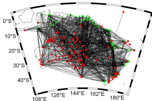
Fig. 2. Ray coverage. Epicentres are plotted as green crosses and stations as red stars.
