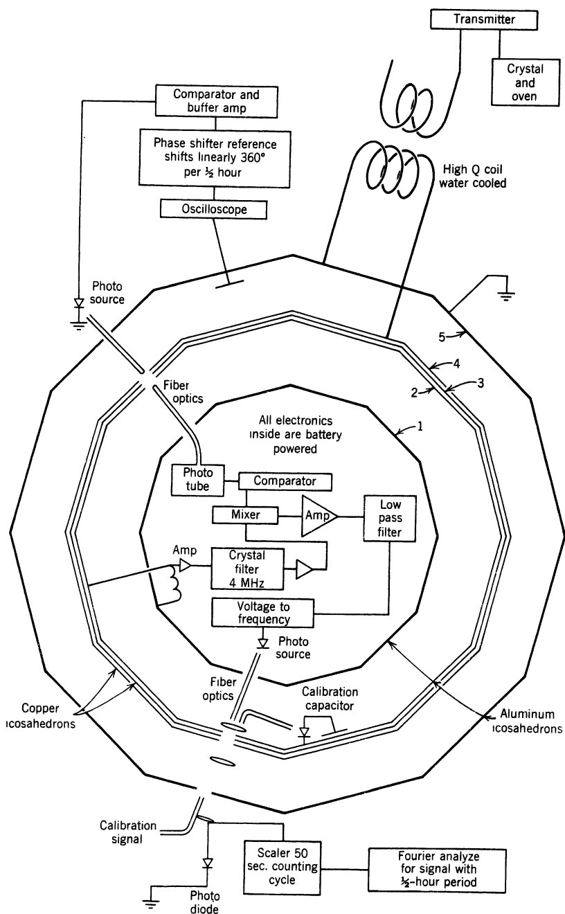
Figure I.2 Schematic diagram of the “Cavendish” experiment of Williams, Faller, and Hill. The concentric icosahedrons are conducting shells. A 4 MHz voltage of 10 kV peak is applied between shells 5 and 4. Shell 4 and its contiguous shells 2 and 3 are roughly 1.5 meters in diameter and contain shell 1 inside. The voltage difference between shells 1 and 2 (if any) appears across the inductor indicated at about 8 o’clock in shell 1. The amplifier and optics system are necessary to extract the voltage information to the outside world. They are equivalent to Cavendish’s system of strings that automatically opened the hinged hemispheres and brought up the pith balls to test for charge on the inner sphere. (Figure reproduced with permission of the authors.)
