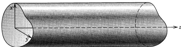
Figure 8.3 Hollow, cylindrical waveguide of arbitrary cross-sectional shape.
