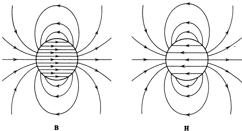
Figure 5.11 Lines of B and lines of H for a uniformly magnetized sphere. The lines of B are closed curves, but the lines of H originate on the surface of the sphere where the effective surface magnetic “charge,” \sigma_M , resides.
