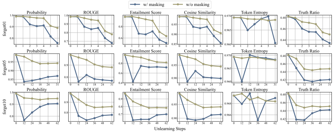
Figure 11: Masking the questions or not when calculating the forget loss in ME+GD on the retain set of forget01, forget05 and forget10 tasks in TOFU.
