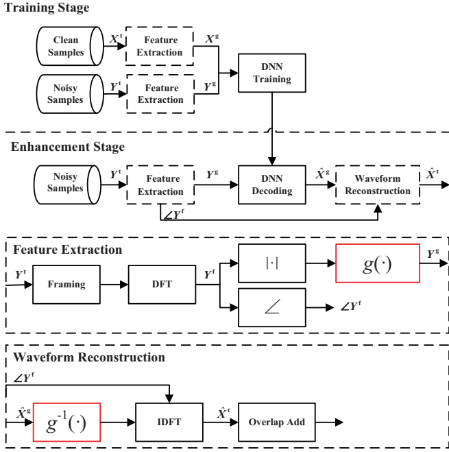
Fig. 1. A block diagram of the DNN-based speech enhancement via the explicit transformation.
