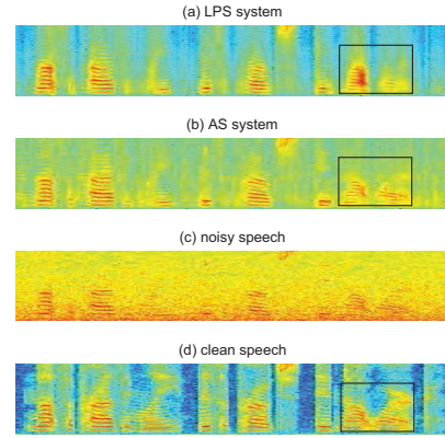
Fig. 2. Spectrogram of an utterance tested with pink noise at -5dB SNR: (a) DNN approach using LPS features (PESQ=1.810, STOI=0.645), (b) DNN approach using AS features (PESQ=1.680, STOI=0.733), (c) noisy speech (PESQ=1.107, STOI=0.573), (d) clean speech.
