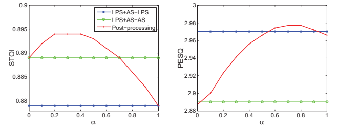
Fig. 5. Average STOI and PESQ performance on 13 unseen noise types across different SNRs.
