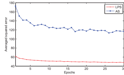
Fig. 3. The comparison of DNN learning curves using averaged squared errors on development set in LPS domain.
