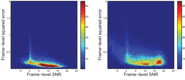
Fig. 4. The comparison of distribution with respect to frame-level squared error and frame-level SNR on the development set in LPS domain after DNN learning for LPS system (left) and AS system (right).
