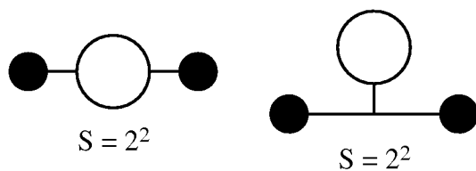
Figure 9.6: All connected diagrams with E = 2 and V = 2 .
