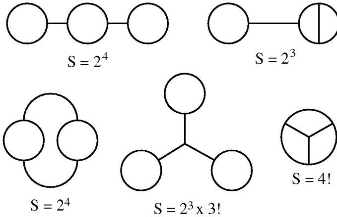
Figure 9.1: All connected diagrams with E = 0 and V = 2 .
