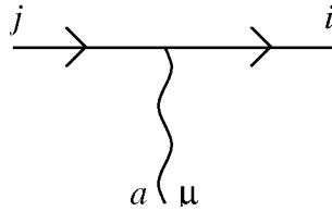
Figure 72.2: The ghost-ghost-gluon vertex in nonabelian gauge theory.
