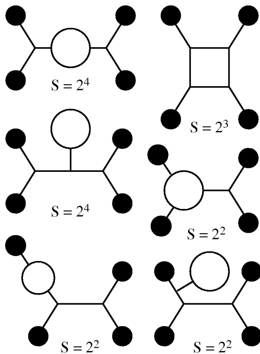
Figure 9.10: All connected diagrams with E = 4 and V = 2 .
