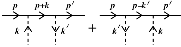
Figure 45.4: Diagrams for e^- \varphi \rightarrow e^- \varphi , corresponding to eq. (45.16).
