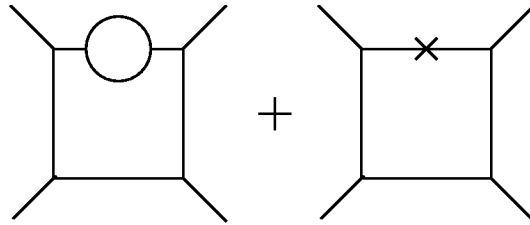
Figure 18.1: The one-loop contribution to \mathbf{V}_4 .
