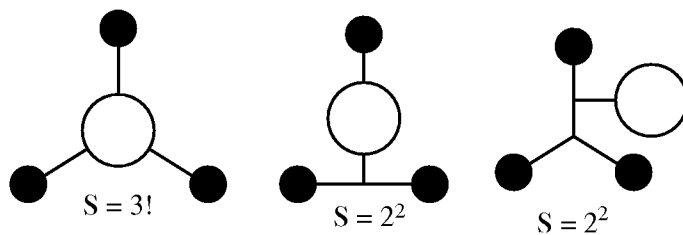
Figure 9.9: All connected diagrams with E = 3 and V = 3 .
