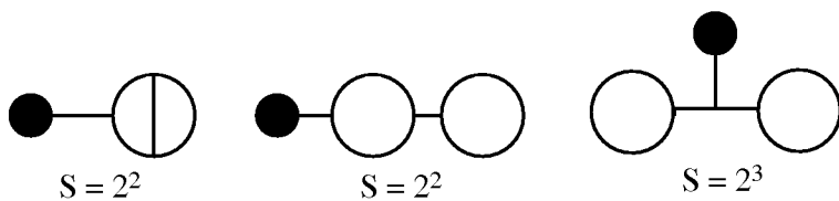
Figure 9.4: All connected diagrams with E = 1 and V = 3 .
