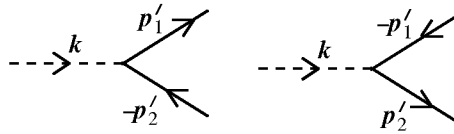
Figure 49.1: Two equivalent diagrams for \varphi \rightarrow \nu\nu .
