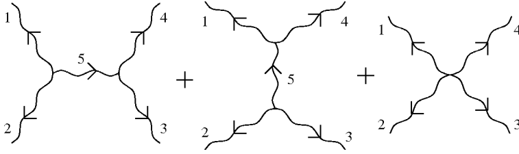
Figure 81.1: Diagrams for the partial amplitude A(1, 2, 3, 4) .
