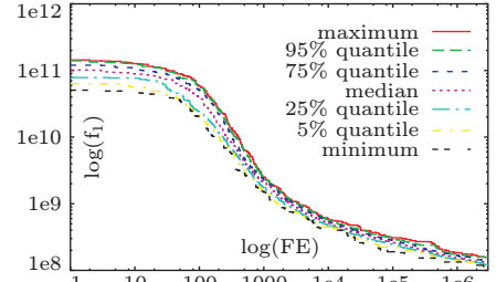
Fig. 3.c: Performance of HC-C on f_1 , dimension = 200.
