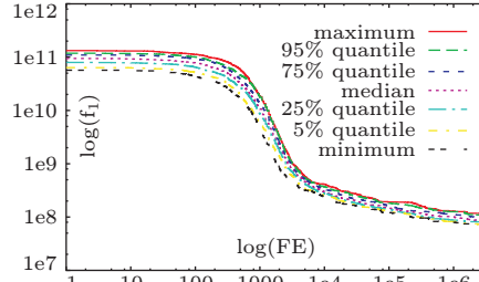
Fig. 3.b: Performance of HC-G on f_1 , dimension = 200.
