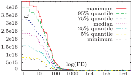
Fig. 3.f: Performance of HC-C on f_4 , dimension = 400.
