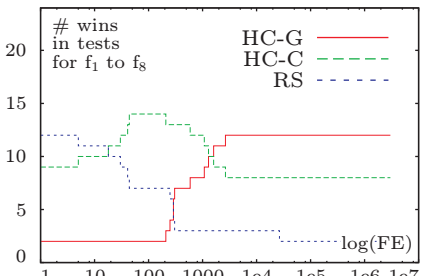
Fig. 3.j: The total test wins in all functions dimension = 200.
