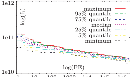
Fig. 3.a: Performance of RS on f_1 , dimension = 200.
