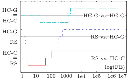
Fig. 3.i: Comparison of the optimizers on f_7 , dimension = 400.
