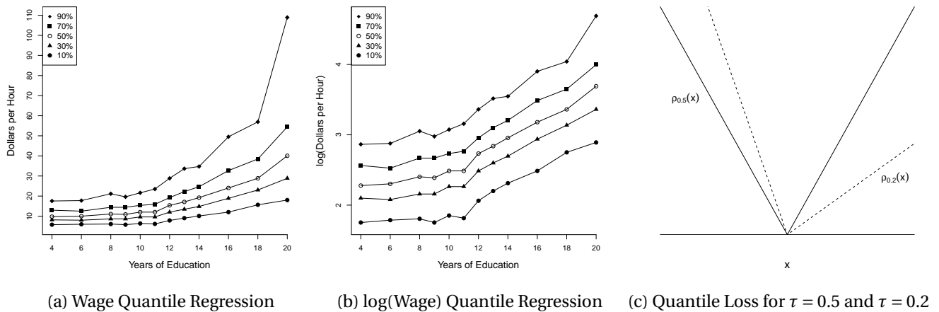
Figure 24.2: Quantile Regressions
