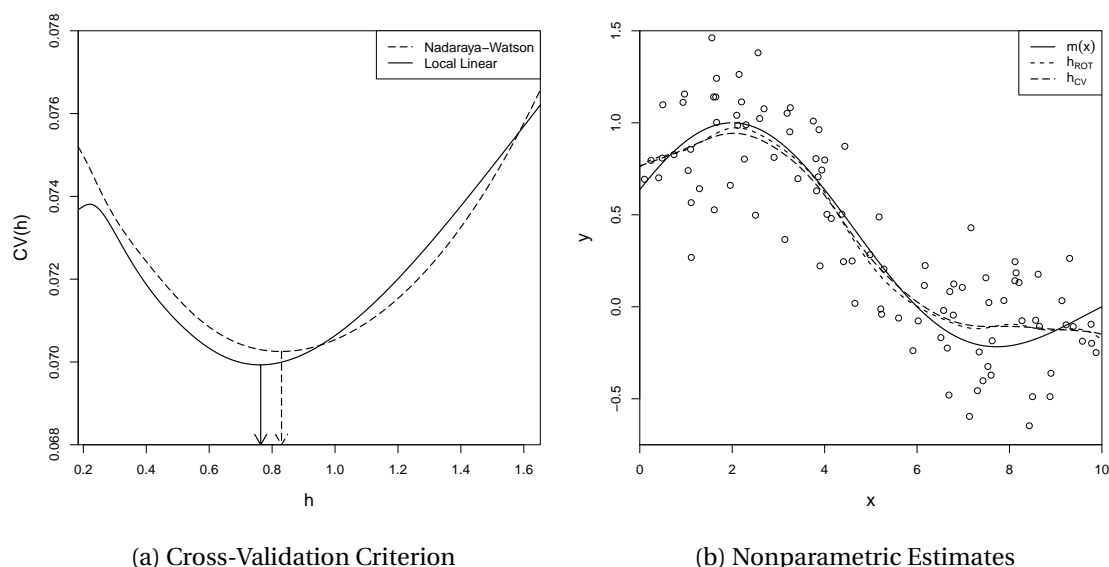
Figure 19.3: Bandwidth Selection
