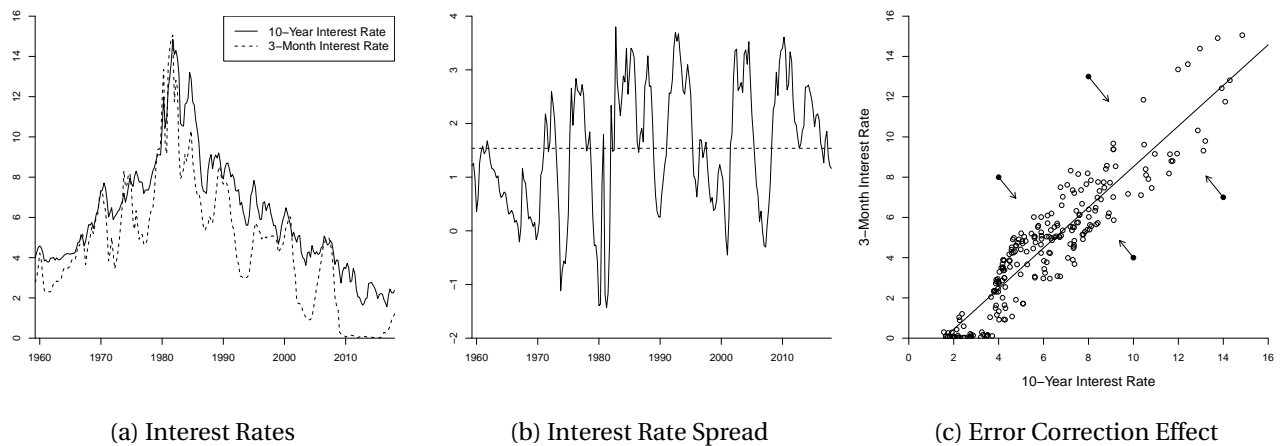
Figure 16.6: Cointegration
