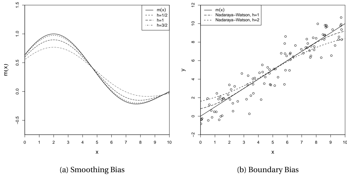
Figure 19.2: Asymptotic Bias
