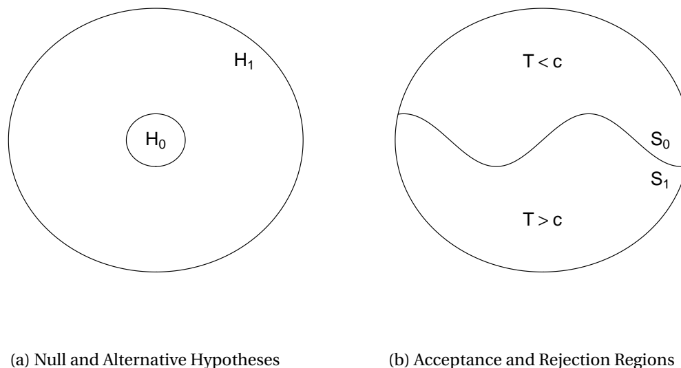
Figure 9.1: Hypothesis Testing
