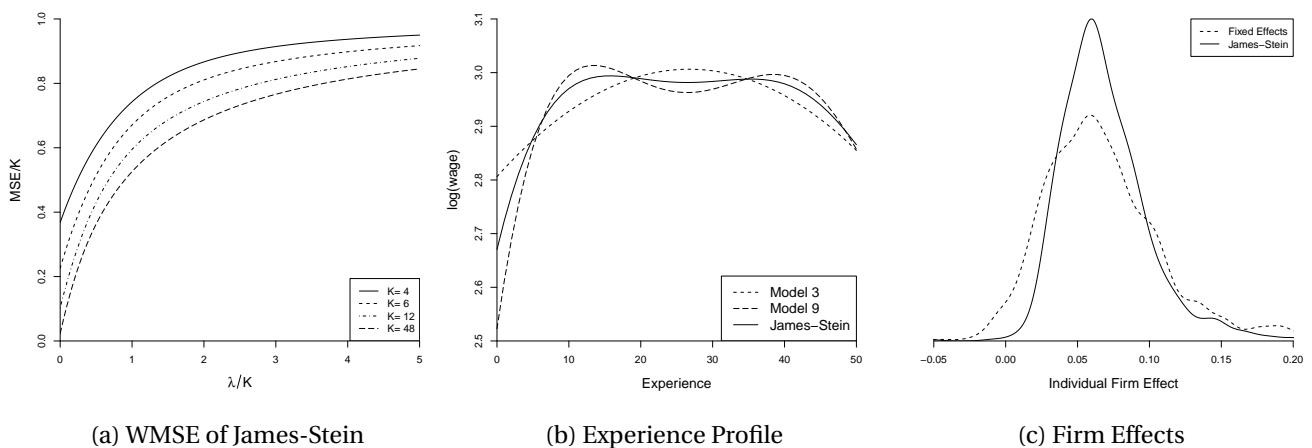
Figure 28.3: James-Stein Estimator
