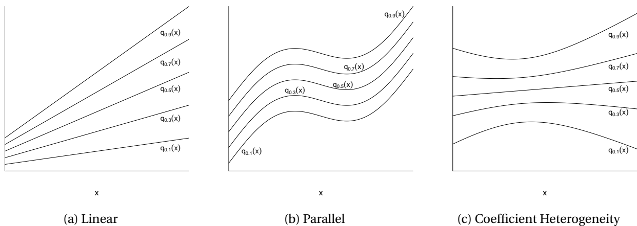
Figure 24.3: Quantile Shapes
