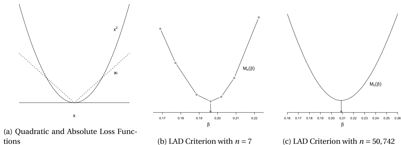
Figure 24.1: LAD Criterion
