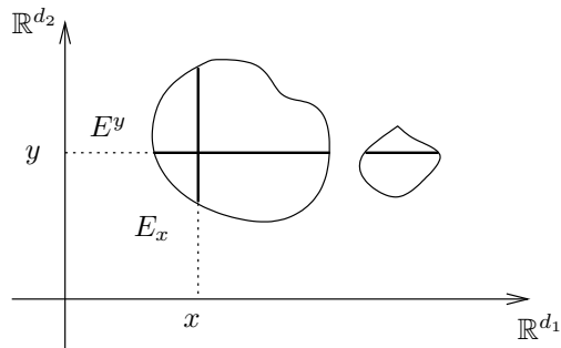
Figure 1. Slices E^y and E_x (for fixed x and y ) of a set E
