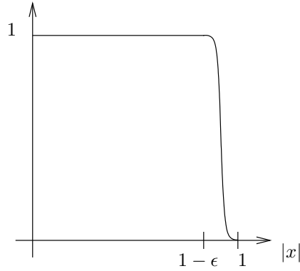
Figure 3. The function \eta_\epsilon^+
